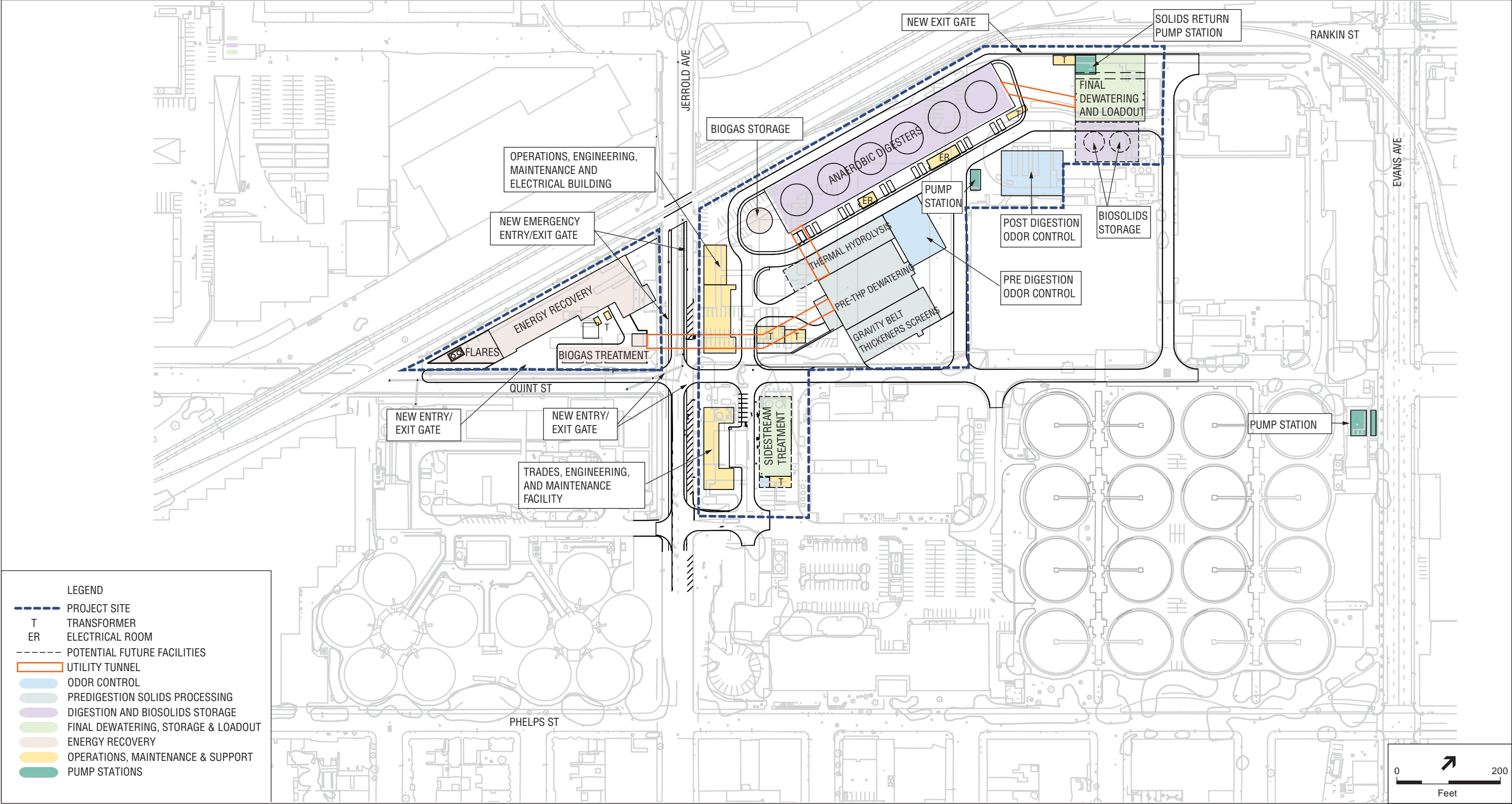
Biosolids Digester Facilities Project Figure 4 Preliminary Site Plan
